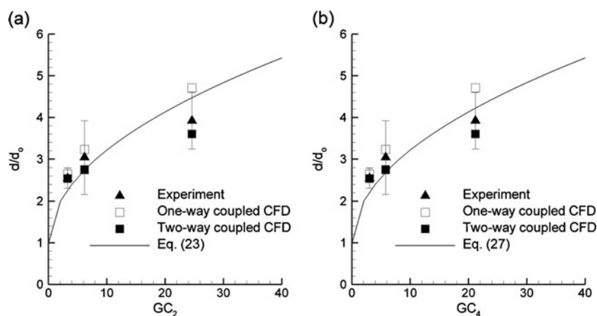
Fig. 7 Comparison of growth ratios determined using the experiments and CFD models with algebraic correlations (a) Eq. 23 and (b) Eq. 27 from Longest and Hindle (12). Relatively good agreement is observed in comparison with Eq. 23, which neglects two-way coupling. Improved agreement is observed for the fully coupled CFD and experimental results with Eq. 27, which does account for two-way coupled growth. It is concluded that the previously developed algebraic correlations can adequately predict aerosol size change for combination drug:excipient submicrometer particles over standard inhalation periods.
