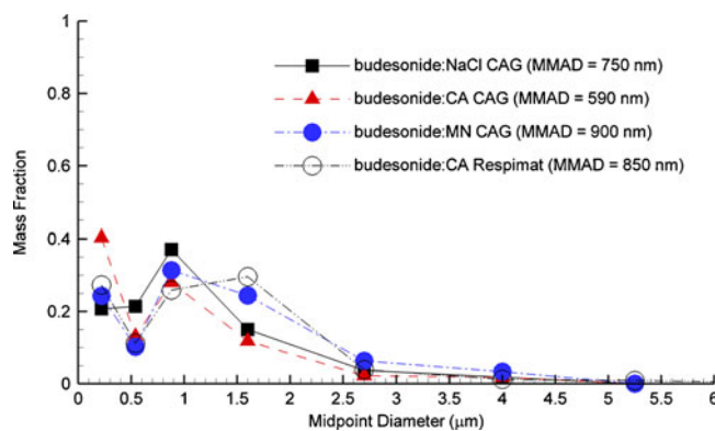
Fig. 2 Aerodynamic size distribution of the initial aerosols from the CAG and Respimat inhalers based on measurements in the ACI. Midpoint diameters are based on the 9 stages of the ACI operated at approximately 30 L/min.
