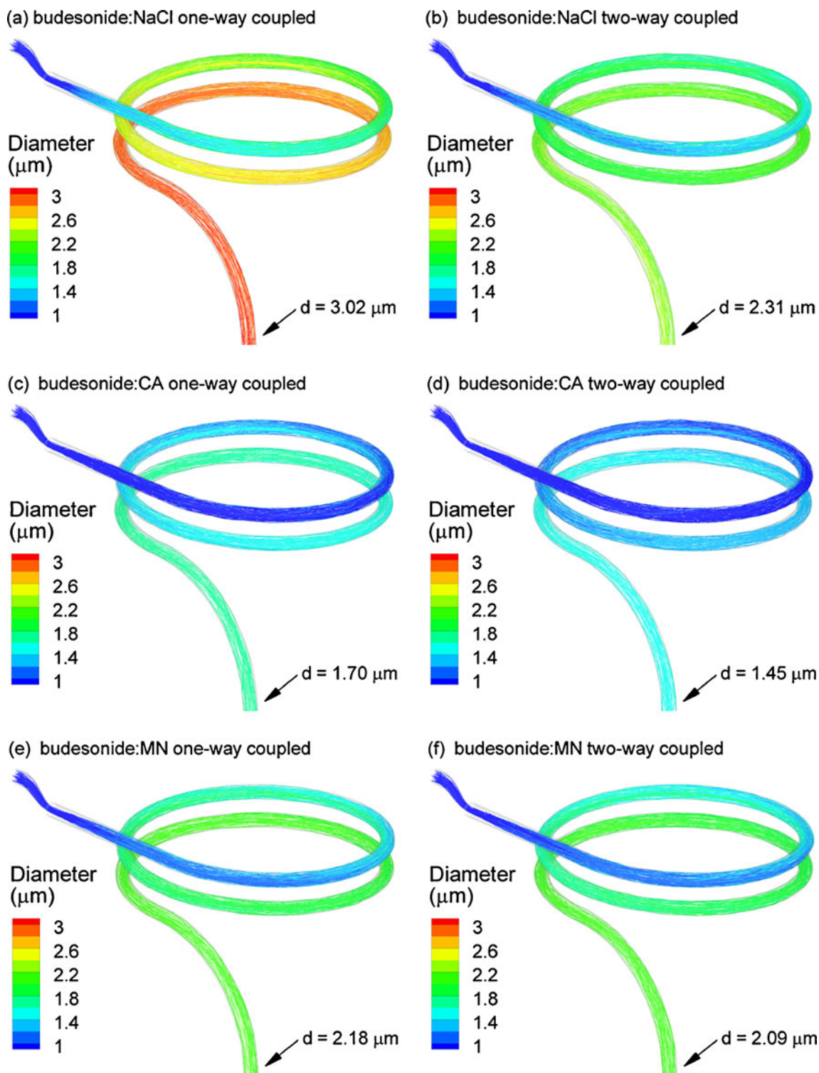
Fig. 4 Particle trajectories colored according to diameter for (a and b) budesonide:NaCl, (c and d) budesonide:CA, and (e and f) budesonide:MN. Left and right panel columns represent one-way and two-way coupled calculations, respectively. For all cases considered, growth appears to occur through a majority of the flow domain with diminishing size increase near the outlet. Coupling effects are greatest for the case of the budesonide:NaCl aerosol and negligible for the budesonide:MN combination.
