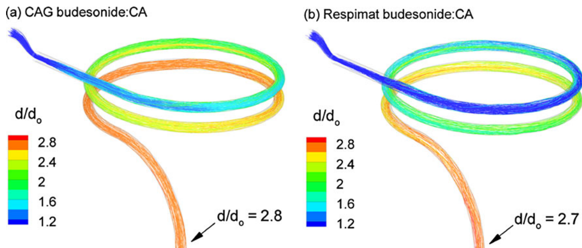
Fig. 5 Particle trajectories contoured based on diameter growth ratio for the budesonide:CA aerosol generated using the (a) CAG and (b) Respimat inhaler. The bolus delivery of the Respimat inhaler appears to reduce the growth ratio by a negligible amount.
